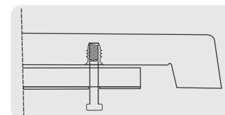
3. Table-Leg Assembly Element 20x40x1.2mm Box Profile 4. AB Bolt
